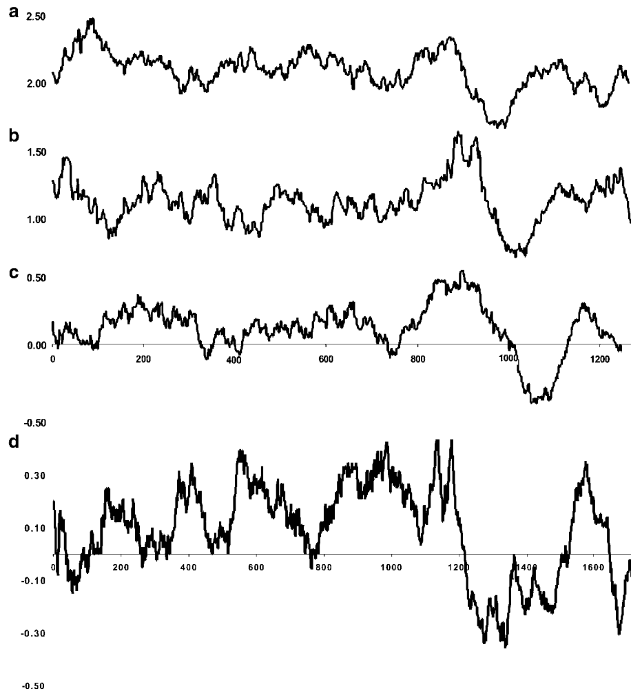
Figure 4 Result of CG-skew analysis of LTR regions, showing the DNA composition computed in a sliding window of 100bp with a step of one base. (a) Pisum sativum RLC-Angela-FJ434420, (b) Medicago truncatula homolog, (c) Oryza sativa RIRE-1, (d) Hordeum vulgare BARE-1. Positive GC-skew values indicate an overrepresentation of G bases, whereas negative GC-skew values represent an overabundance of C bases.
